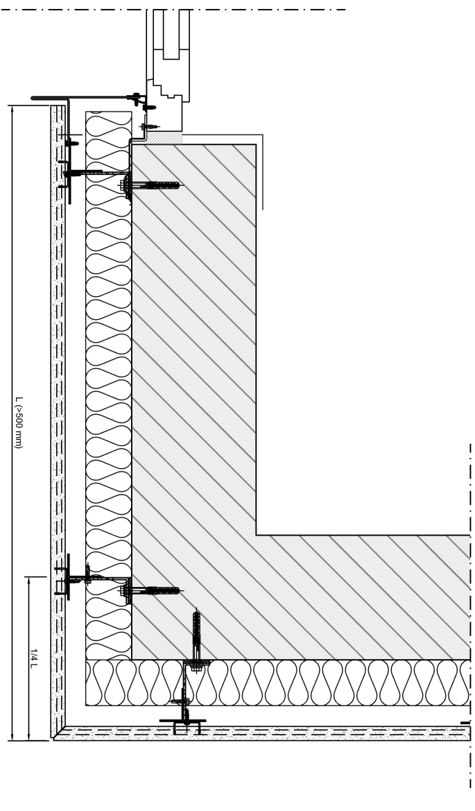
D1 - joint with joint profile
