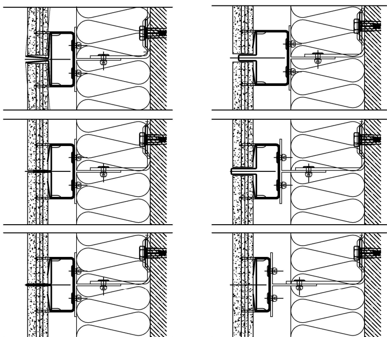
TON_ADS_Joint profiles
