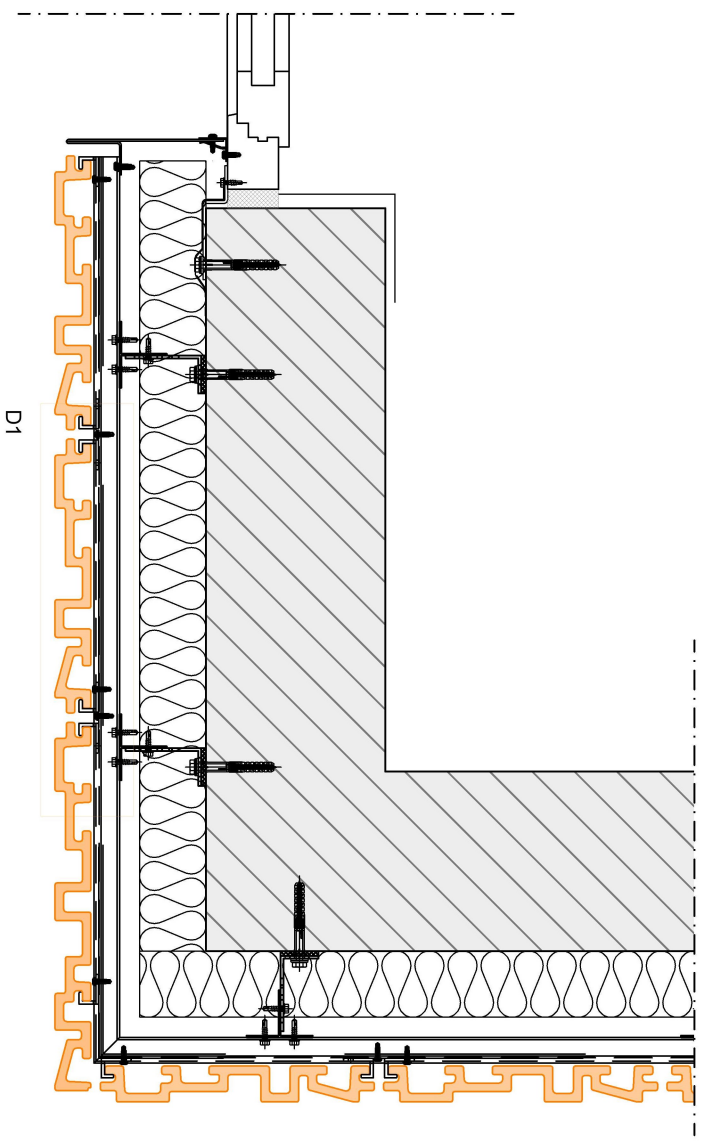
D1 - Fixing of facade elements
