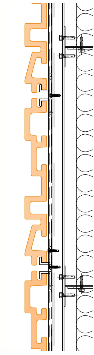
D1 - Fixing of facade elements
