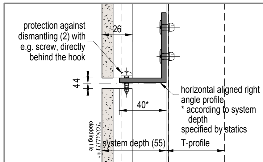
vertikal detail of protection against dismantling (2)
